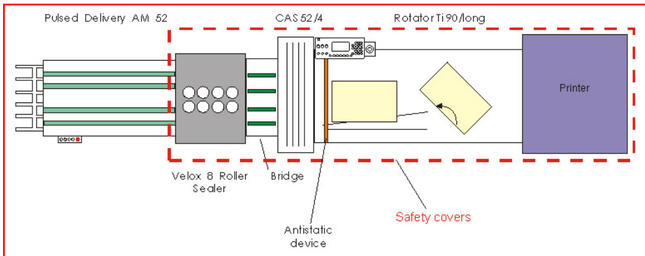
System-Layout - Folding system online with sealer
